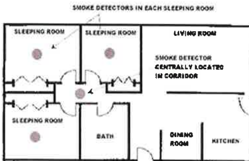
LOCATION OF SMOKE DETECTORS WITHIN A RESIDENCE
